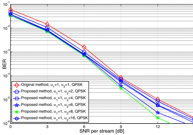
Fig. 4. The simulated BER performance RCI-VP algorithm with different value of \alpha_2 (left: QPSK modulation; right: 16QAM, 64QAM modulations)
