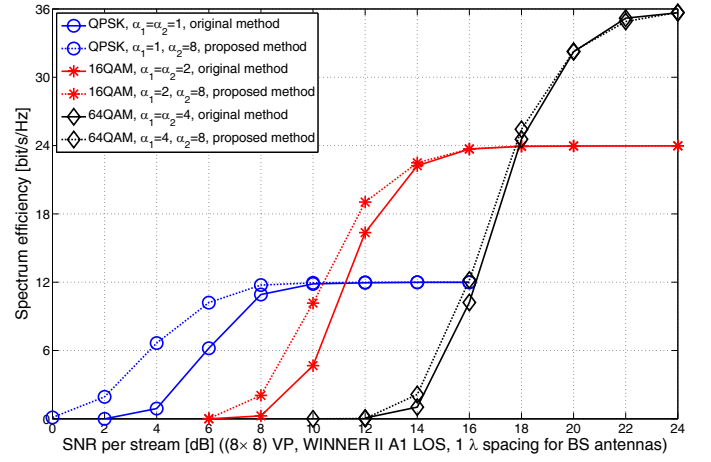
Fig. 6. The spectrum efficiency performance comparison of RCI-VP algorithm with and without dual regularization parameters over A1 LOS MIMO channel (1 \lambda spacing for BS antennas).
