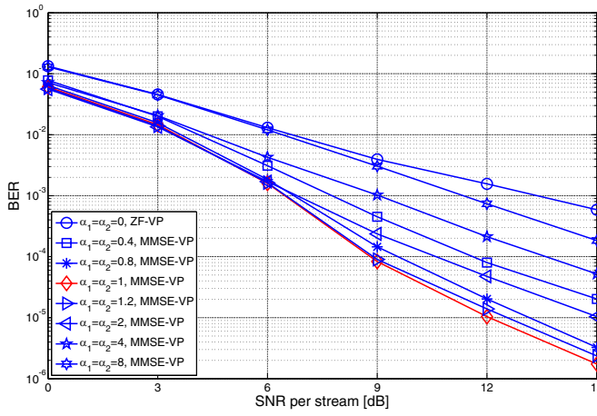
Fig. 3. The simulated BER performance of RCI-VP algorithm when \alpha_1 = \alpha_2 (left: QPSK modulation; right: 16QAM, 64QAM modulations)
