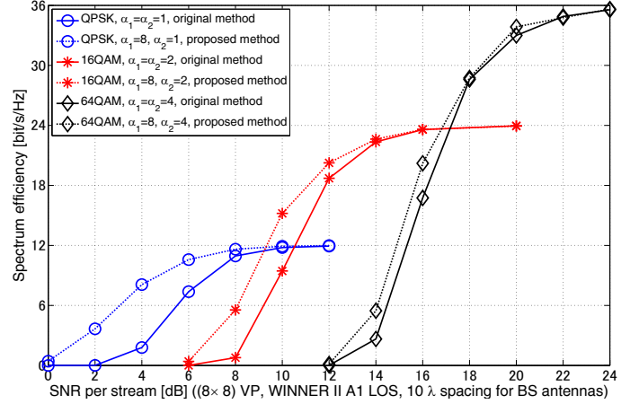
Fig. 7. The spectrum efficiency performance comparison of RCI-VP algorithm with and without dual regularization parameters over A1 LOS MIMO channel (10 \lambda spacing for BS antennas).
