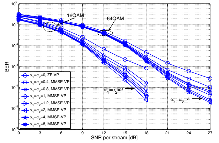
Fig. 3. The simulated BER performance of RCI-VP algorithm when \alpha_1 = \alpha_2 (left: QPSK modulation; right: 16QAM, 64QAM modulations)
