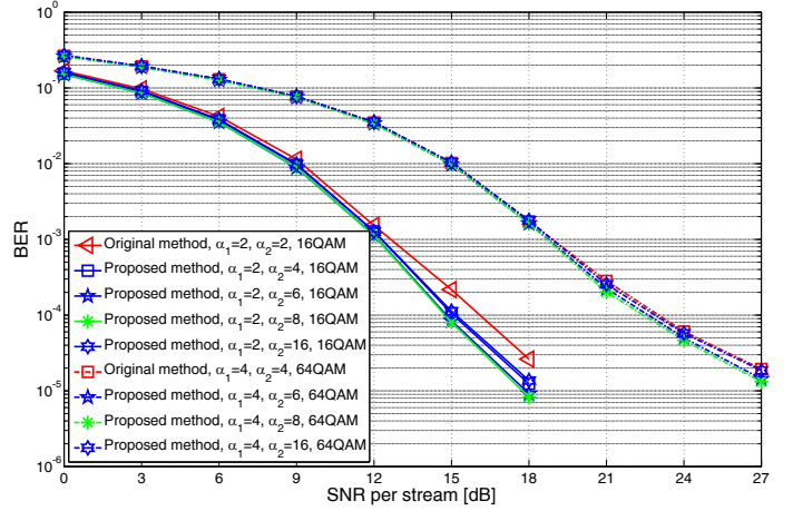
Fig. 4. The simulated BER performance RCI-VP algorithm with different value of \alpha_2 (left: QPSK modulation; right: 16QAM, 64QAM modulations)
