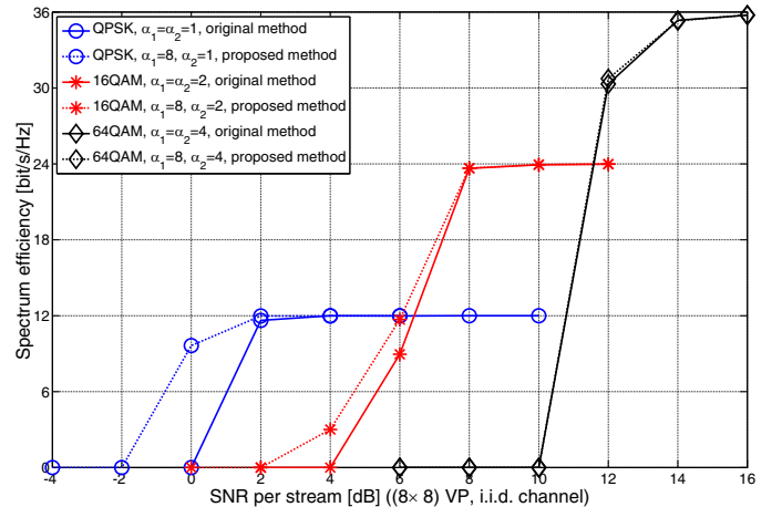
Fig. 5. The spectrum efficiency performance comparison of RCI-VP algorithm with and without dual regularization parameters over i.i.d. MIMO channel.
