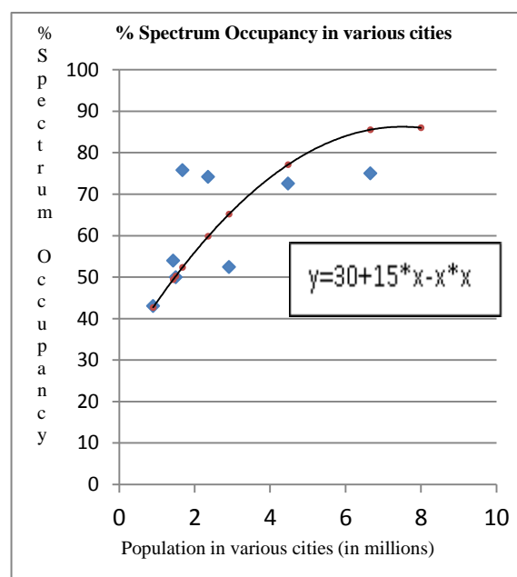
Fig. 4. Population Spectrum Graph
