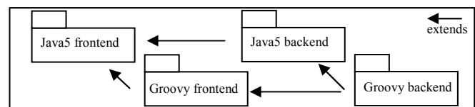
Figure 3. JGroovy: Groovy extension components
