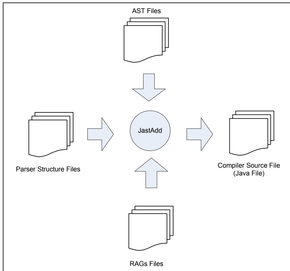
Figure 9. JastAdd compiler construction system
