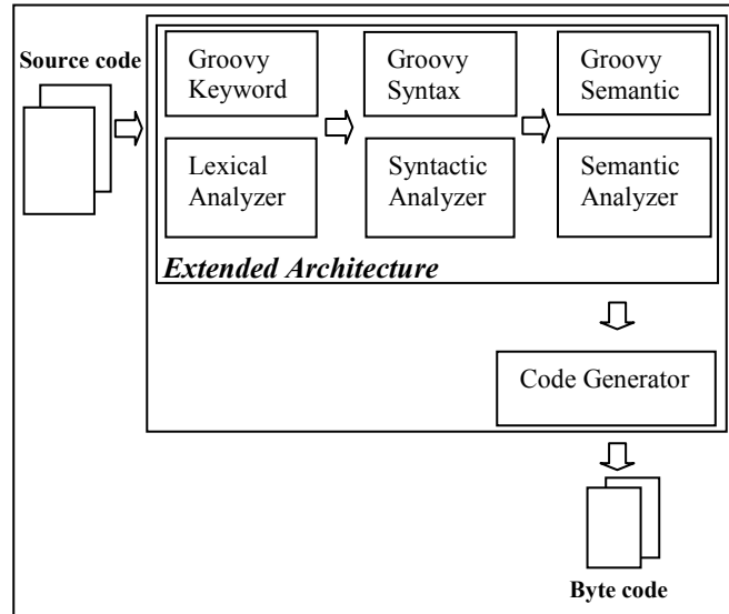
Figure 1. JGroovy compiler achitecture
