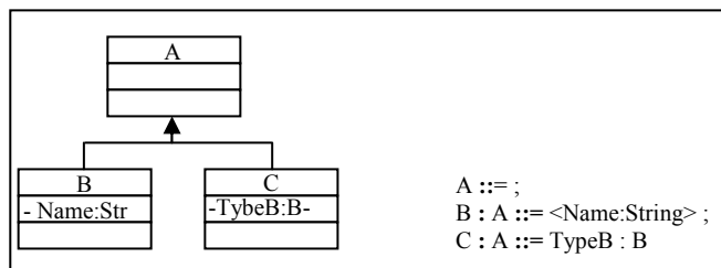
Figure 7. Class heirachy of AST
