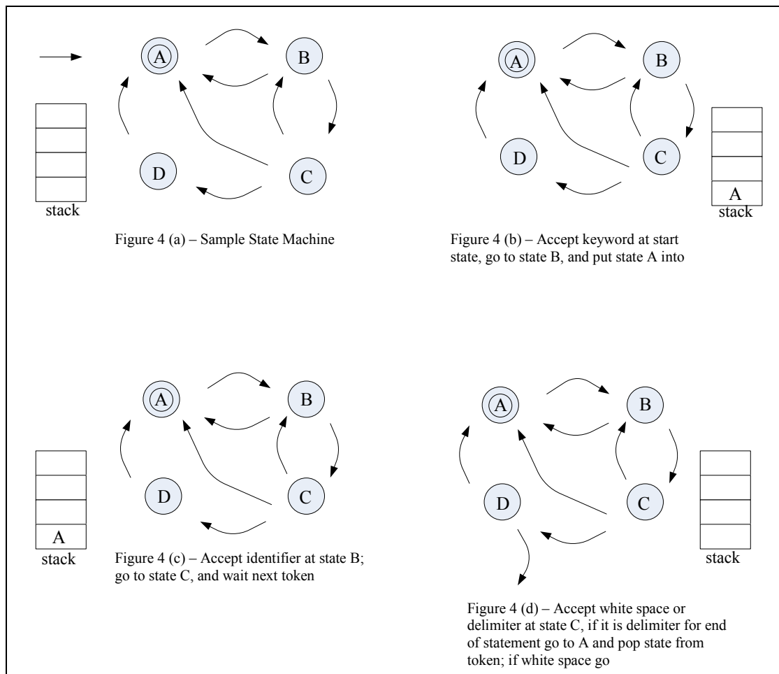
Figure 4. Stack-Machine Scanner Architecture
