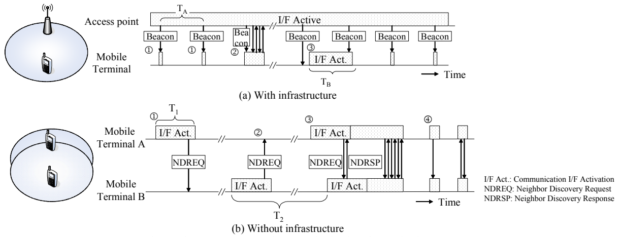
Fig. 1. Discovery process and communication interface activation
