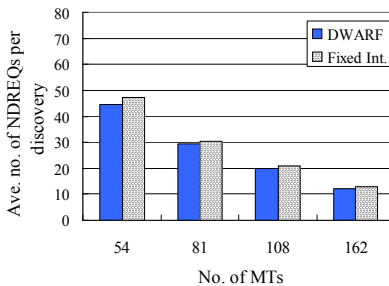
(a) Pause duration: 0 – 120 [s]
