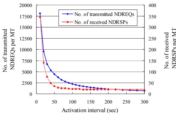
(b) No. of transmitted NDREQs and received NDRSPs Fig. 5. Preliminary experimental results
