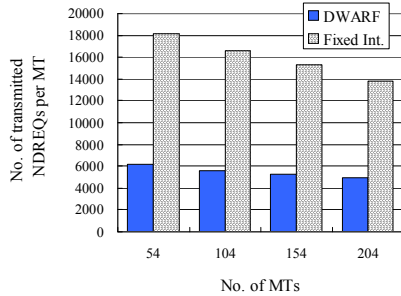
(a) The number of transmitted NDREQs
