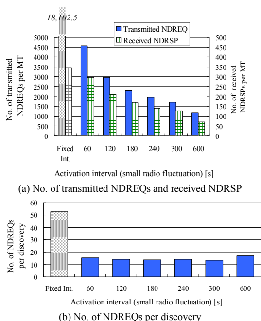
Fig. 9 Result of DWARF at various intervals (in small radio fluctuation)
