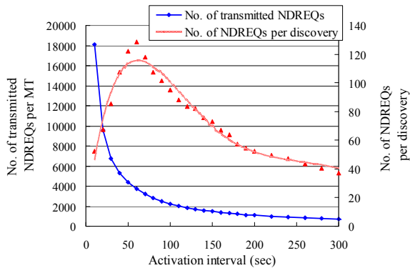
(a) No. of transmitted NDREQs and required NDREQs per discovery
