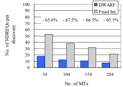
(c) The number of NDREQs per discovery
