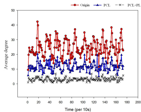
Figure 11. The distribution of average degree in normal traffic.
