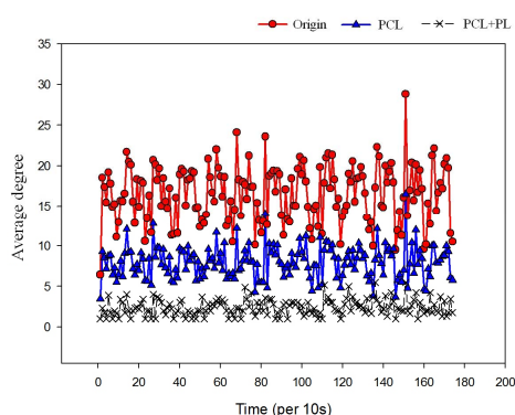
Figure 13. The distribution of average degree in sparse traffic.
