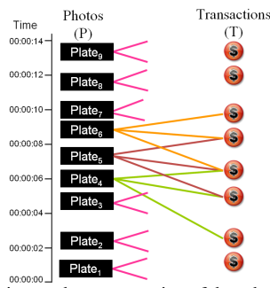
Figure 4. A bipartite graph representation of the relation between image data and transaction data.
