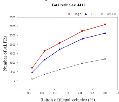
Figure 8. The number of ALPRs in congested traffic.
