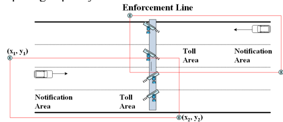
Figure 1. Virtual toll zone configuration in VPS system.
