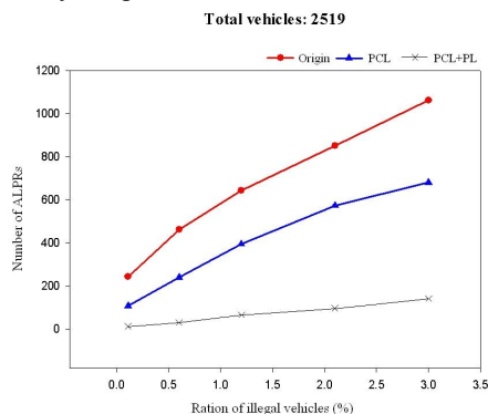
Figure 12. The number of ALPRs in sparse traffic.
