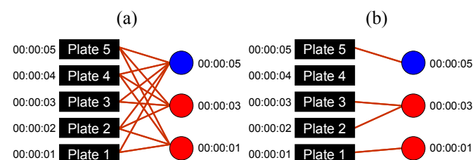
Figure 7. (a) Initial graph. (b) After eliminate the unnecessary edges.
