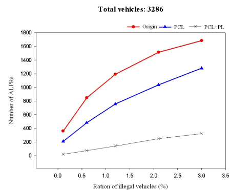
Figure 10. The number of ALPRs in normal traffic.
