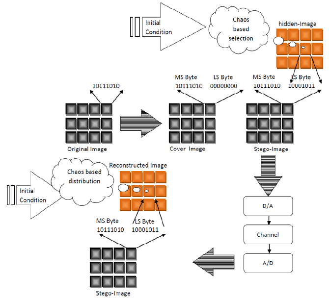
Figure 1. The proposed steganography algorithm
