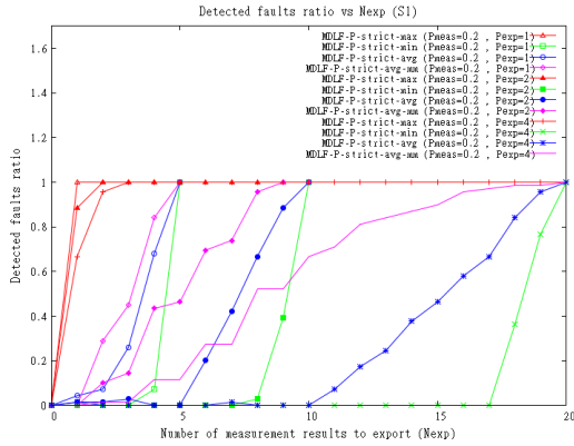
Fig. 3. Detected faults ratio vs N_{exp} when FDLM-P-strict is used.
