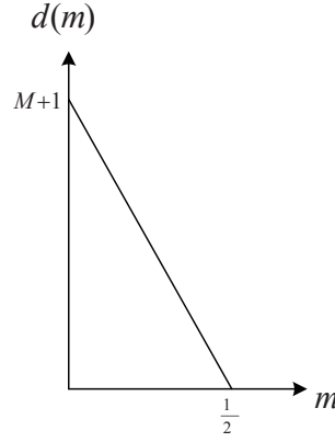
Fig. 2: Diversity-multiplexing tradeoff for the max-generalized-mean (MGM) selection criterion in the AF-OR.
