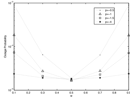
Fig. 5: Simulated outage probability of the AF-OR under the max-generalized-mean (MGM) selection criterion when SNR = 30 dB. Number of relays M = 4 .
