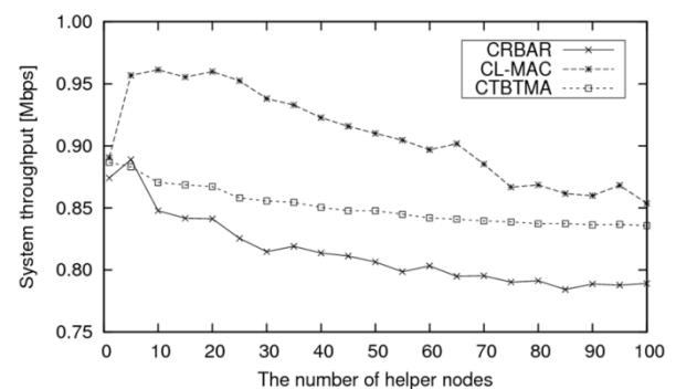
Figure 2. System throughput of three schemes as a function of the number of helper nodes
