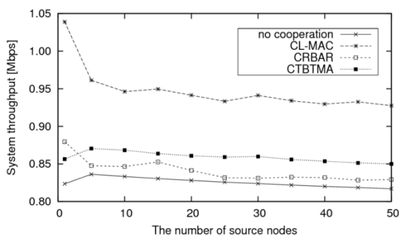
Figure 3. Comparison of system throughput as a function of the number of source nodes
