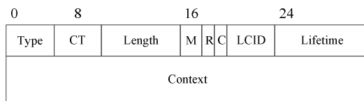
Figure 8. Context Notification Option
