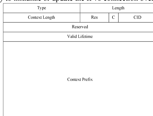
Figure 4. 6LoWPAN Context Option format
