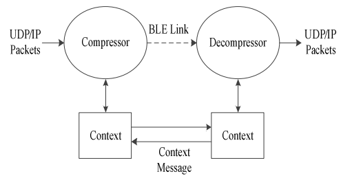
Figure 6. Header Compression System Diagram
