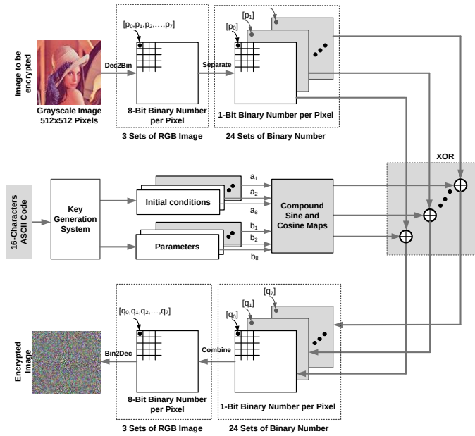
Figure 1. Proposed encryption algorithms using the compound sine and cosine chaotic maps.
