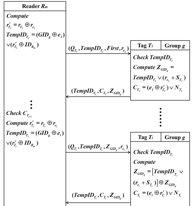
Figure 2. Main authentication phase of the proposed protocol
