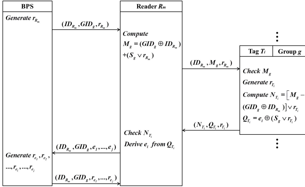
Figure 1. Tag acquisition phase of the proposed protocol
