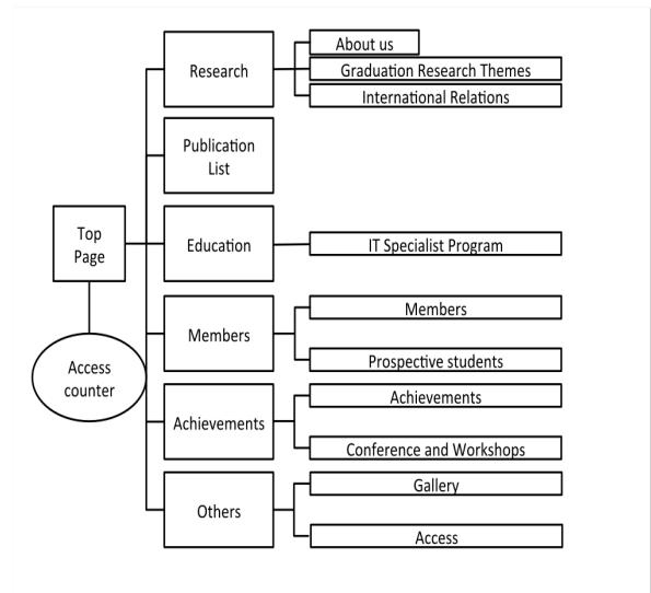
Figure 1. Website architecture
