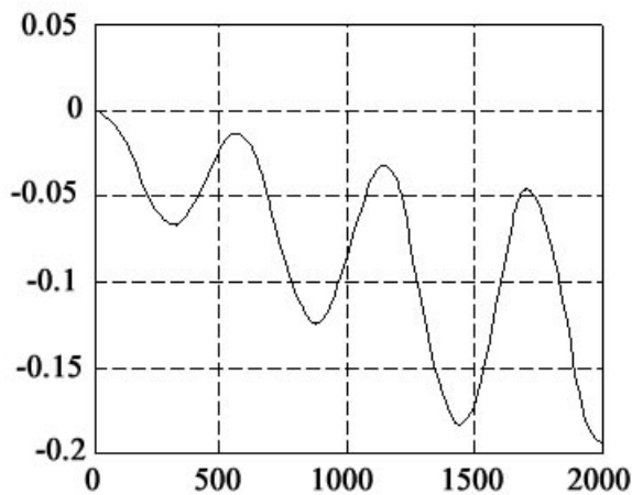
Figure 2. Angular displacement with in the y-direction
