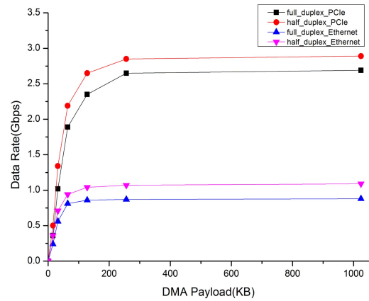
Figure 7. Performance of UPI system
