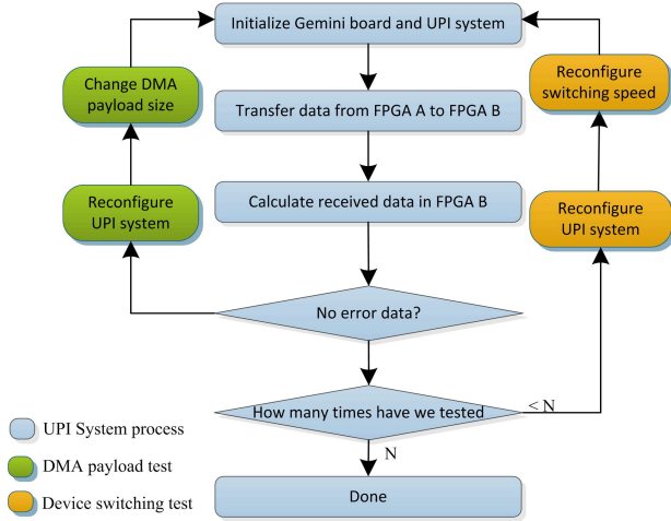
Figure 6. Flow chart of UPI testing program
