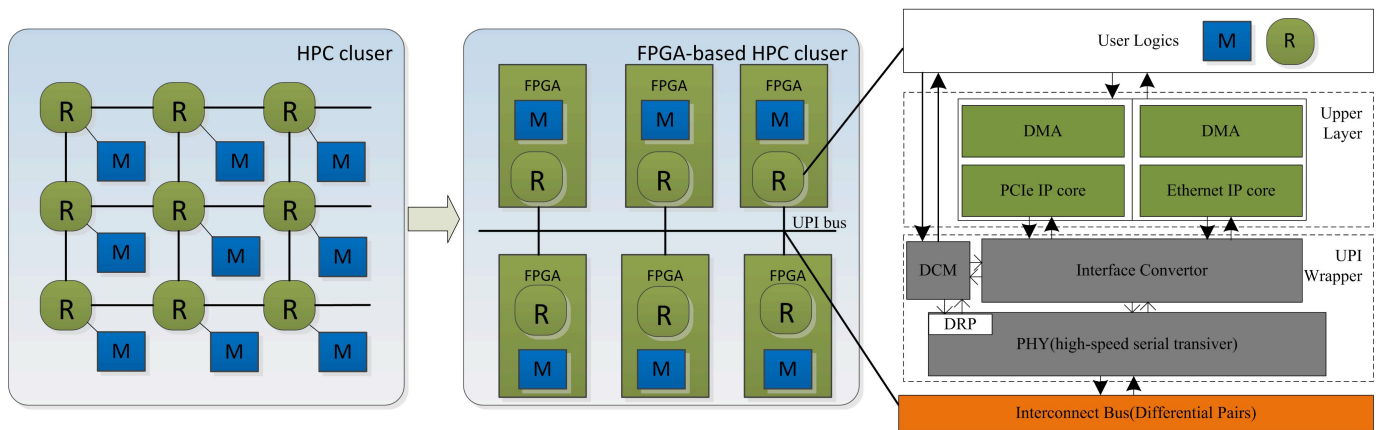
Figure 1. Hardware structure of UPI system
