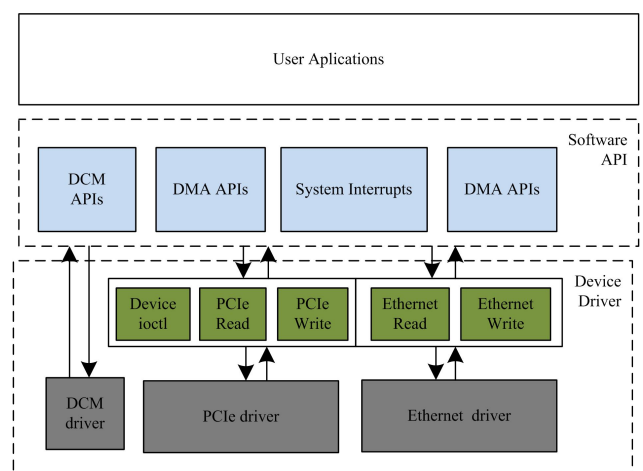
Figure 2. Software structure of UPI system
