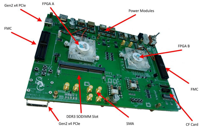
Figure 4. “Gemini” Prototype Verification Board
