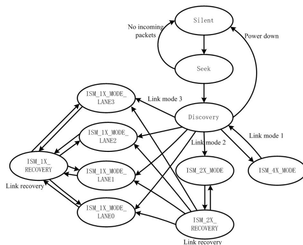
Figure 3. DRP control module link training state machine
