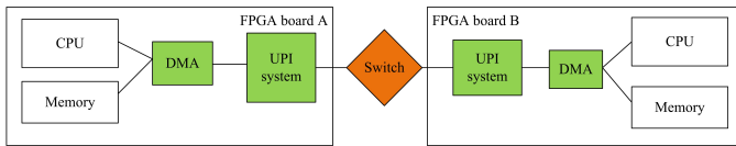
Figure 5. Structure of FPGA-based verification system
