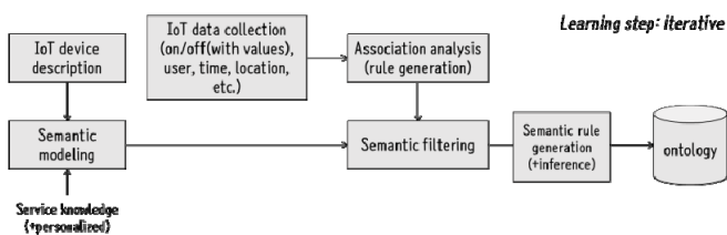
Figure 6. Rule learning step
