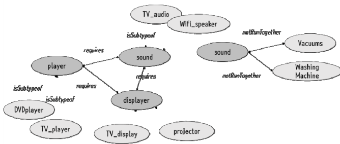
Figure 5. Semantic model example for an auto-device configuration
