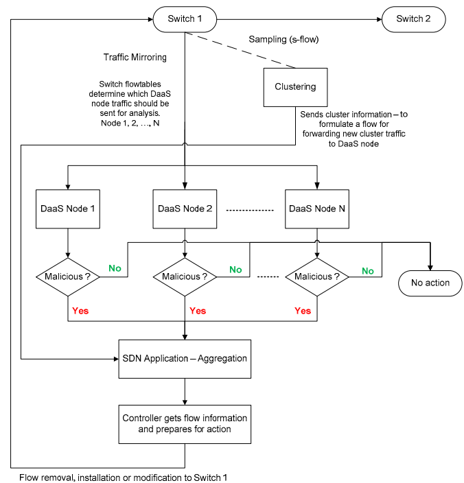
Figure 4. Flowchart for approach 2 for DaaS in SDN
