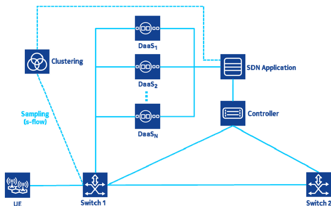
Figure 3. Approach 2 for DaaS in SDN
