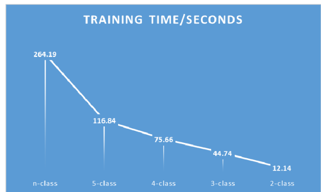
Figure 4. Change in training time as the number of classes are decreased
