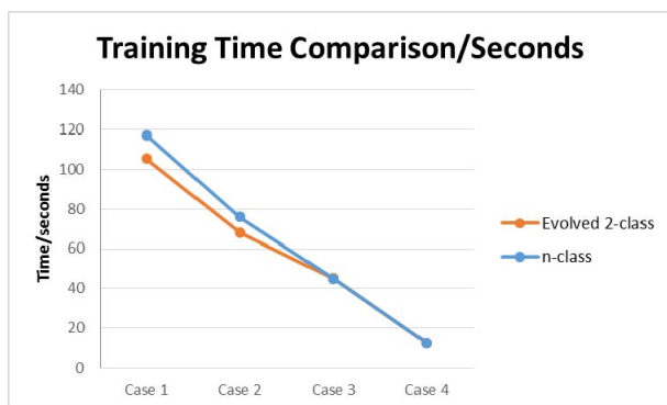
Figure 5. Training time comparison between n-class and evolved 2-class
