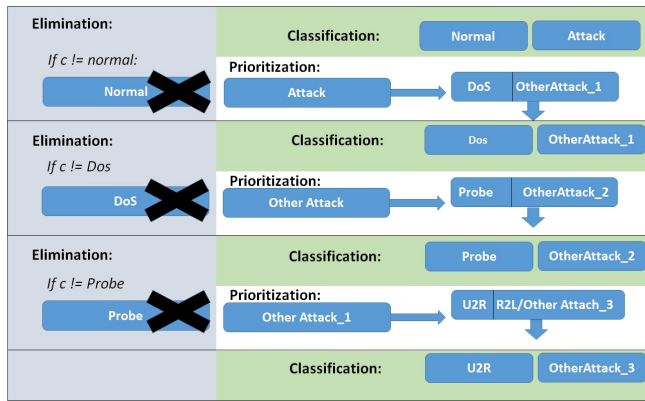
Figure 2. Evolving ANN based 2-class IDS mechanism
