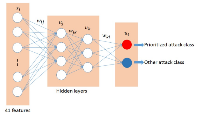
Figure 1. ANN based 2-class IDS mechanism
