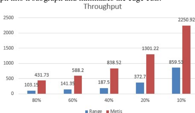
Figure 2. Throughput when multiple-tuple transaction rate varies
