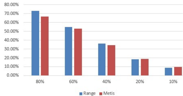
Figure 3. Distributed transaction when multiple-tuple transaction rate varies
