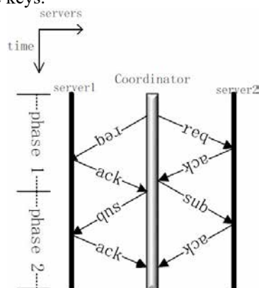
Figure 1. A typical two phase commit example in modern OLTP database
