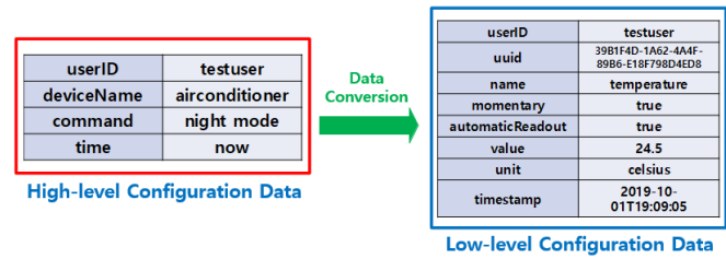
Figure 5. Example of converting data
