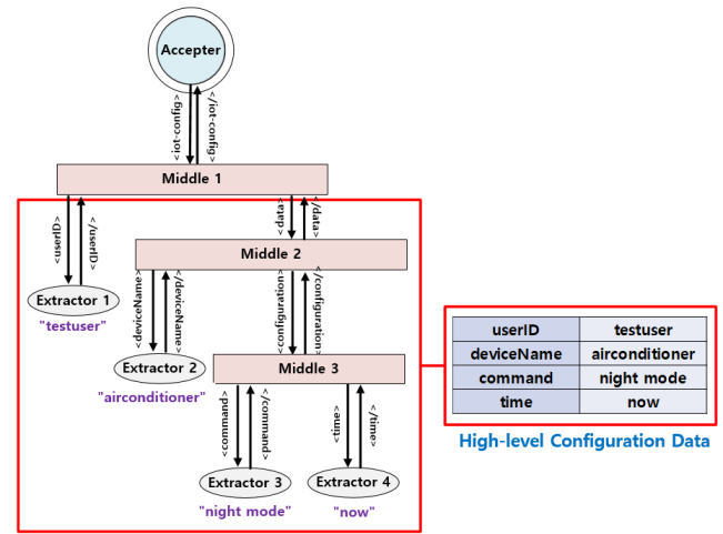
Figure 4. Example of Extractor schema
