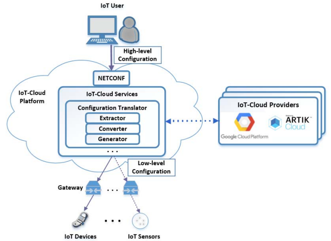
Figure 1. The Architecture of an IoT device configuration translator
