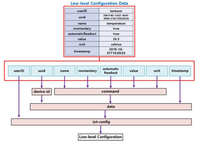
Figure 6. Example of generator schema
