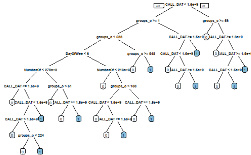
Fig. 3. Decision Tree for the CART Model
