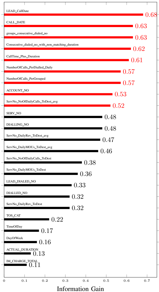
Fig. 1. Information Gain of each Feature
