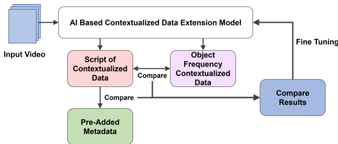
Figure 2. Process of Model Fine-Tuning
