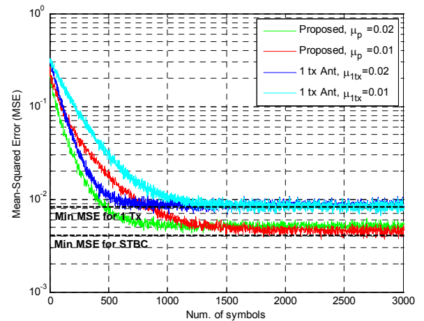
Fig. 2. MSE learning curves for the proposed scheme and general single transmit antenna scheme
