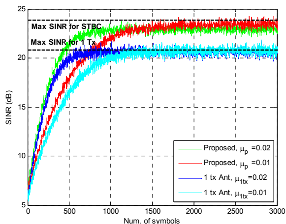
Fig. 3. SINR comparison between the proposed scheme and single antenna case
