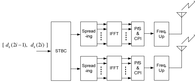
Fig. 1. Transmitter structure for MC-CDMA system employing STBC
